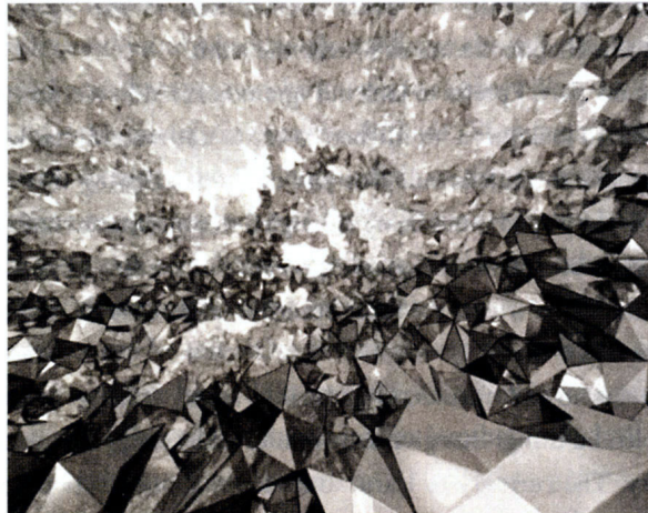
Figure 13.1 An intuitive representation of quantum gravity
